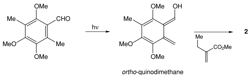
ortho -quinodimethane
