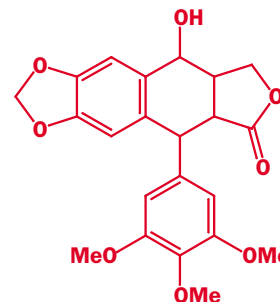
the anti-cancer compound podophyllotoxin
