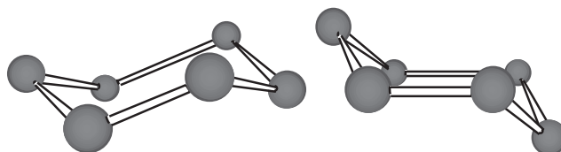
the carbon skeleton for cyclohexane
