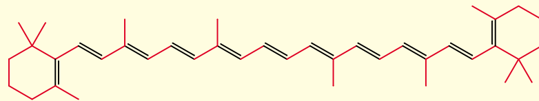
\beta -carotene, the red pigment in carrots and other vegetables
