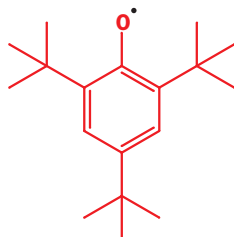
dark blue solid m.p. 97°C
