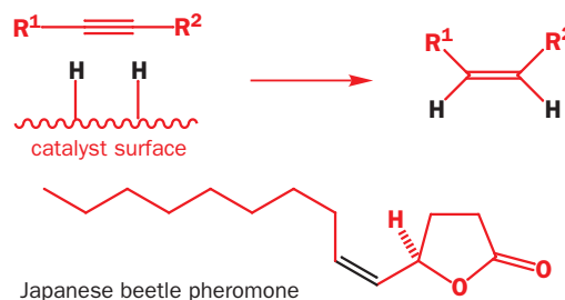
Japanese beetle pheromone
