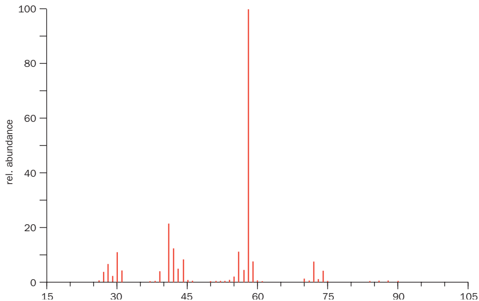
the electron impact mass spectrum of an industrial emulsifier
