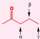
\alpha,\beta -unsaturated ketone
