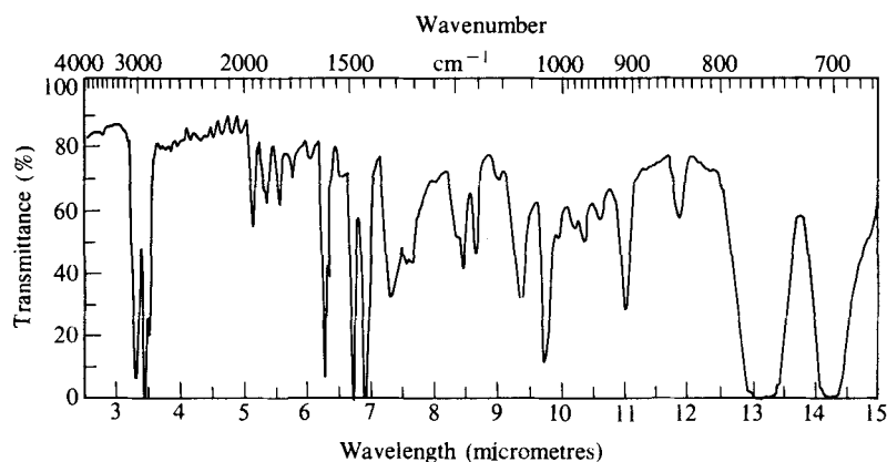
Fig. 19.1 The infrared spectrum of polystyrene.
