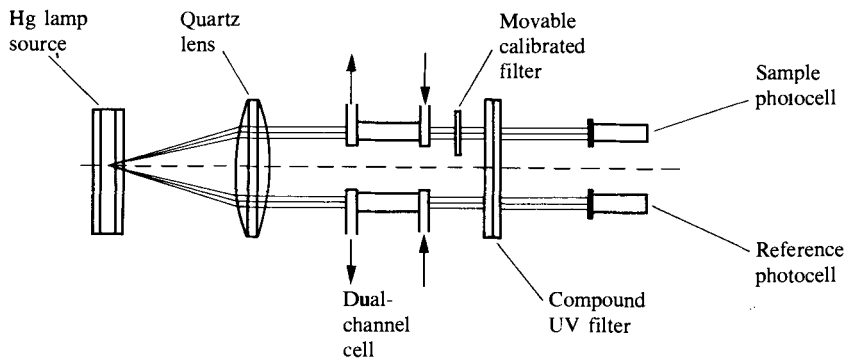
Fig. 8.5 Block diagram of a double-beam UV detector.
