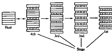
Fig. 16.4 Staging in graphite intercalation compounds, C_{12n}K . Addition of potassium proceeds through n = 4, 3, 2, \dots to the limit in stage 1: C_{12n}K \rightarrow C_6K . [From Whittingham, M. S.; Dines, M. B. Surv. Prog. Chem. 1980, 9, 55. Reproduced with permission.]
