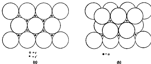
Fig. 4.12 (a) Sites created by layer 1 and available to accept atoms in layer 2. (b) Covering all t sites by atoms in the second layer, making the r' sites (relabelled o ) unavailable for occupancy by close-packed atoms.
