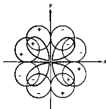
Fig. 11.25 \pi overlap of t_{2g} LGOs with a metal t_{2g} ( d_{xy} ) orbital. There are two additional sets perpendicular to the one shown.
