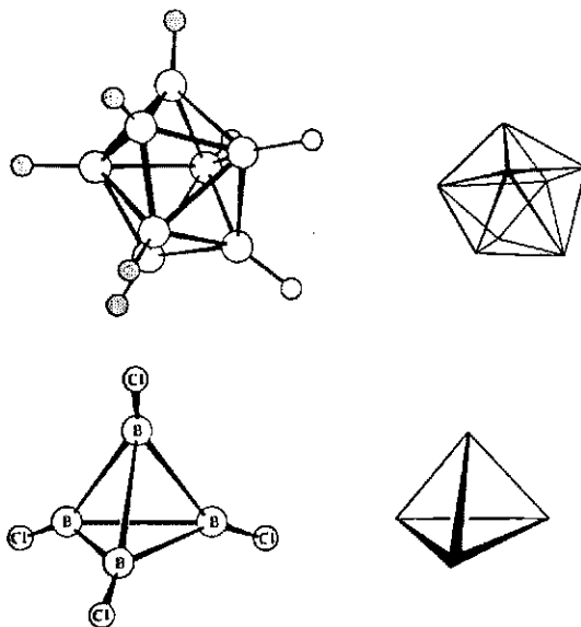
Fig. 16.48 (a) The structure of the [B_8H_8]^{2-} anion compared to an idealized dodecahedron. [From Guggenberger, L. J. Inorg. Chem. 1969, 8, 2771. Reproduced with permission.] (b) Molecular structure of B_3Cl_4 compared to an idealized tetrahedron. [From Muettietries, E. L. The Chemistry of Boron and Its Compounds ; Wiley: New York, 1967. Reproduced with permission.]
