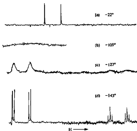
Fig. 6.30 ^{19}\text{F} NMR spectra of a solution of \text{PCl}_2\text{F}_2 in isopentane at various temperatures. All of the fluorine resonances are doublets from ^{31}\text{P} - ^{19}\text{F} coupling. (a) At -22^\circ\text{C} only a single doublet is observed, indicating that all of the fluorine atoms are equivalent. (b) At -109^\circ\text{C} this resonance disappears. (c) At -127^\circ\text{C} two new absorptions appear. (d) At -143^\circ\text{C} two types of fluorine atoms are seen: a doublet of doublets at low field (two axial F's) and a doublet of triplets at higher field (one equatorial F). [From Holmes, R. R.; Carter, R. P., Jr.; Peterson, G. E. Inorg. Chem. 1964, 3, 1748-1754. Reproduced with permission.]
