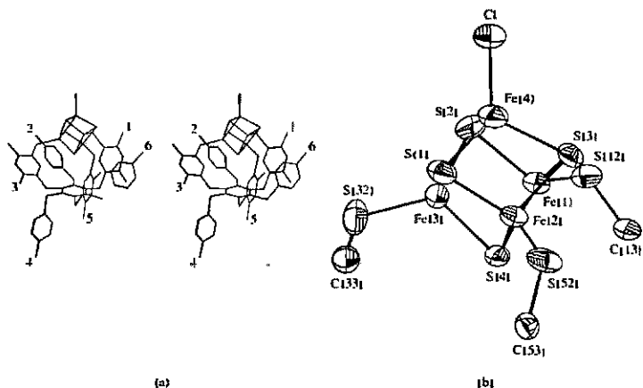
Fig. 19.14 Model compound for a cubane-type \text{Fe}_4 cluster with a trithiol ligand. (a) Stereoview of [\text{Fe}_4\text{S}_4(\text{trithiol})\text{L}'] ; (b) close-up view of the Fe-S cluster. [From Stack, T. D. P.; Holm, R. H. J. Am. Chem. Soc. 1988, 110, 2484-2494. Reproduced with permission.]
