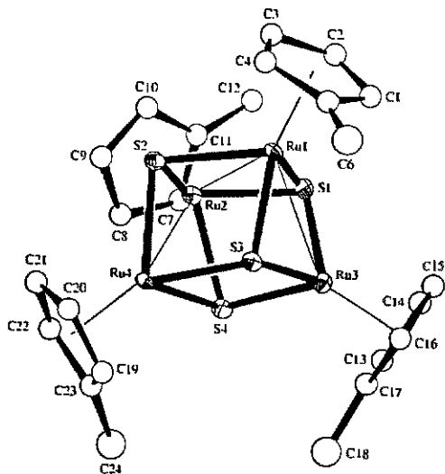
Fig. 15.56 Structure of [(\text{CH}_3\text{C}_5\text{H}_4)_4\text{Ru}_4\text{S}_4]^{2+} . [From Houser, E. J.; Amarasekera, J.; Rauchfuss, T. B.; Wilson, S. R. J. Am. Chem. Soc. 1991, 113, 7440-7442. Reproduced with permission.]
