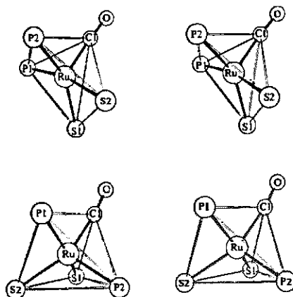
Fig. 12.14 Stereoviews of the inner coordination spheres about the central ruthenium atom in the orange (top) and violet (bottom) isomers of [(C_6H_5)_3P]_2Ru(CO)[(CF_3)_2C_2S_2] . [From Bernal, I.; Clearfield, A.; Ricci, J. S., Jr. J. Cryst. Mol. Struct. 1974, 4, 43-54. Reproduced with permission.]
