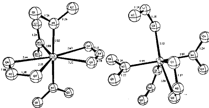
Fig. 12.52 Two forms of the [\text{Cu}(\text{NO}_2)_5]^{2-} ion. All bond distances in angstroms. [From Klanderman, K. A.; Hamilton, W. C.; Bernal, I. Inorg. Chem. Acta 1977, 23, 117-129. Reproduced with permission.]
