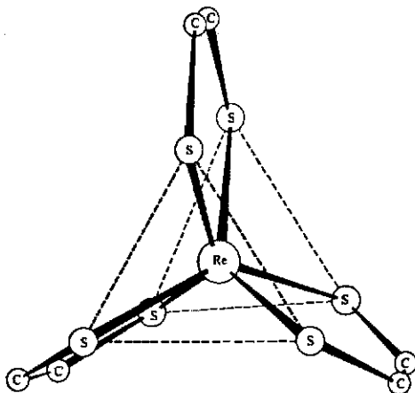
Fig. 12.17 Structure of [\text{Re}(\text{S}_2\text{C}_2\text{Ph}_2)_3] . The phenyl rings have been omitted for clarity. [From Eisenberg, R.; Ibers, J. A. Inorg. Chem. 1966, 5, 441-446. Reproduced with permission.]
