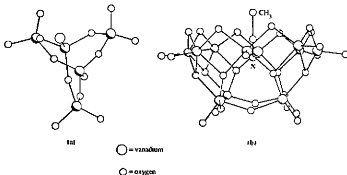
Fig. 16.12 Structures of two oxoanions of vanadium prepared from nonaqueous solvents. (a) [V_5O_{14}]^{3-} . (b) [CH_3CNCV_{12}O_{32}]^{4-} . (The acetonitrile molecule is suspended in the basket denoted by the symbol C.) [From Day, V. W.; Klemperer, W. G.; Yaghi, O. M. J. Am. Chem. Soc. 1989, 111, 4518 and 5959. Reproduced with permission.]
