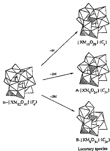
Fig. 16.18 Examples of the polyoxometalate \alpha\text{-[XM}_{12}\text{O}_{40}]^{4-} ion losing both one metal fragment \text{[XM}_{11}\text{O}_{39}] and three metal fragments (isomers A\text{-[XM}_{9}\text{O}_{34}] and B\text{-[XM}_{9}\text{O}_{34}] ). The structures formed (called lacunary structures) have vacant sites which can be filled by other metal fragments. [From Pope, M. T.; Müller, A. Angew. Chem. Int. Ed. Engl. 1991, 30, 34–48. Reproduced with permission.]
