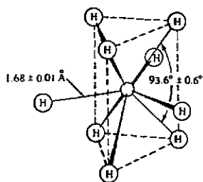
Fig. 12.39 Stereoviews of the structure of (a) \text{trans-SmI}_2[\text{O}(\text{CH}_2\text{CH}_2\text{OCH}_3)_2]_2 and (b) \text{cis-SmI}_2[\text{O}(\text{CH}_2\text{CH}_2\text{OCH}_3)_2]_2 . [From Sen, A.; Chebott, V.; Rheingold, A. L. Inorg. Chem. 1987, 26, 1821–1823. Reproduced with permission.]
