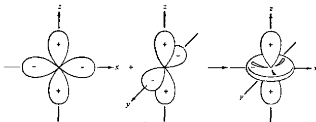
Fig. 11.5 Representation of the d_{z^2} orbital as a linear combination of d_{z^2-x^2} and d_{z^2-y^2} orbitals. The d_{z^2} label is actually shorthand notation for d_{2z^2-x^2-y^2} .
