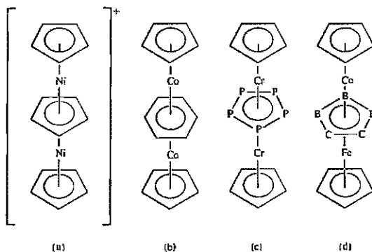
Fig. 15.37 Some known "triple deckers" containing cyclopentadienyl ligands.
