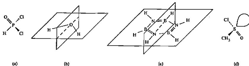
Fig. 3.2 Molecules with and without mirror planes: (a) dichlorophosphine oxide has a single mirror plane (the sheet of the paper) that reflects the two chlorine atoms into each other; (b) water has two mirror planes: one which bisects the H—O—H angle, the other that lies in the plane defined by the H—O—H angle; (c) borazine has four mirror planes: three are of the vertical type shown, and the fourth is the plane of the ring; (d) methylsulfinyl chloride has no plane of symmetry. Note that the lone pair is not experimentally observed in the latter compound, but has been added to rationalize the molecular structure.
