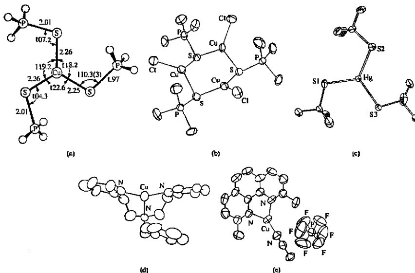
Fig. 12.1 Three-coordinate complexes: (a) \text{Cu}[\text{SP}(\text{Me})_3]^+ ; (b) [\text{Cu}(\text{SP}(\text{CH}_3)_2)\text{Cl}]_3 ; (c) [\text{Hg}(\text{SBu})_3]^- ; (d) [\text{C}_6\text{H}_5\text{CH}_2\text{N}(\text{CH}_2\text{CH}_2\text{C}_6\text{H}_4\text{N})_2\text{Cu}]^+ ; (e) [(\text{CH}_3\text{CN})\text{CuN}_2\text{C}_{12}\text{H}_8(\text{CH}_3)_2]\text{PF}_6 . Carbon atoms are unmarked and hydrogen atoms have been omitted. [From Eller, P. G.; Corfield, P. W. R. Chem. Commun. 1971, 105-106. Tiethof, J. A.; Stalick, J. K.; Meek, D. W. Inorg. Chem. 1973, 12, 1170-1174. Tiethof, J. A.; Hetey, A. T.; Meek, D. W. Inorg. Chem. 1974, 13, 2505-2509. Watton, S. P.; Wright, J. G.; MacDonnel, F. M.; Bryson, J. W.; Sabat, M.; O'Halloran, T. V. J. Am. Chem. Soc. 1990, 112, 2824-2826. Blackburn, N. J.; Karlin, K. D.; Concannon, M.; Hayes, J. C.; Gultneh, Y.; Zubieta, J. Chem. Commun. 1984, 939-940. Munakata, M.; Maekawa, M.; Kitagawa, S.; Matsuyama, S.; Masuda, H. Inorg. Chem. 1989, 28, 4300-4302. Reproduced with permission.]
