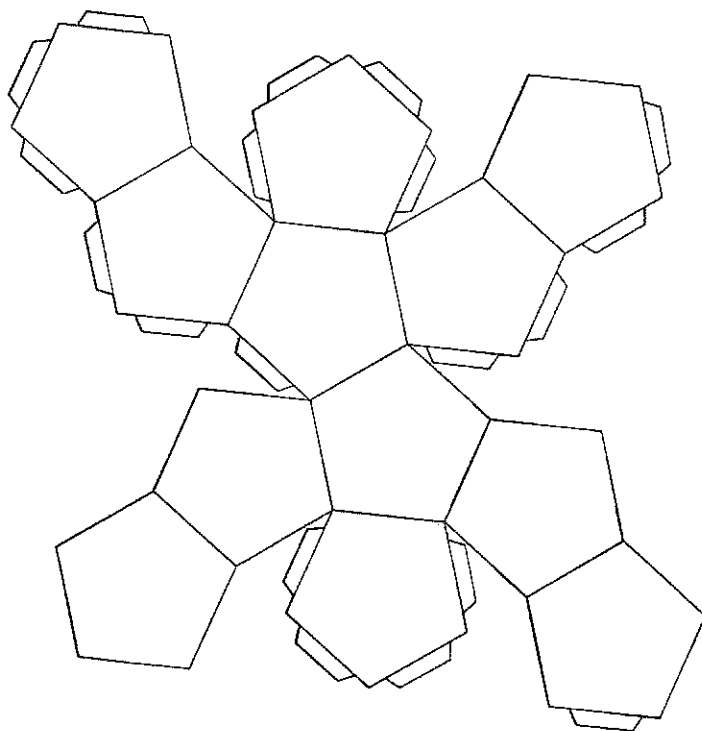
Pentagonal Dodecahedron
