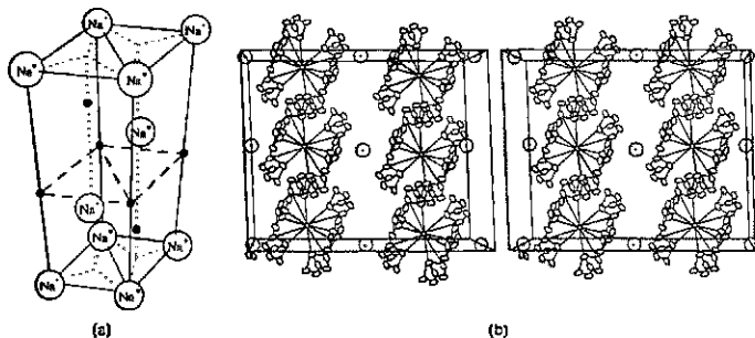
Fig. 12.50 (a) Packing of [\text{NaC222}]^+ (large circles) and \text{Na}^- (small solid circles) ions in cryptandsodium sodide. (b) ORTEP stereo packing diagram of bis(18-crown-6)cesium electride. The anionic hole centers are indicated by the symbol \text{O} . [From Tehan, F. J.; Barnett, B. L.; Dye, J. L. J. Am. Chem. Soc. 1974, 96, 7203; Dawes, S. B.; Ward, D. L.; Huang, R. H.; Dye, J. L. J. Am. Chem. Soc. 1986, 108, 3534–3535. Reproduced with permission.]
