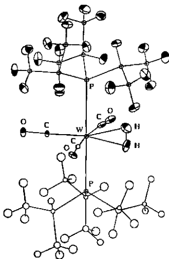
Fig. 15.11 Structure of \text{Mo}(\text{CO})_5(\text{PPR}_3)_2\text{H}_2 , the first nonclassical dihydrogen complex to be discovered. [From Kubas, G. J. Acc. Chem. Res. 1988, 21, 120-128. Reproduced with permission.]
