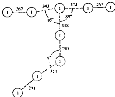
Fig. 17.9 A portion of the structure of the "enneiodide" ion found in \text{Me}_2\text{NI}_9 . The shortest distance between this moiety and the next is only 349 pm.
