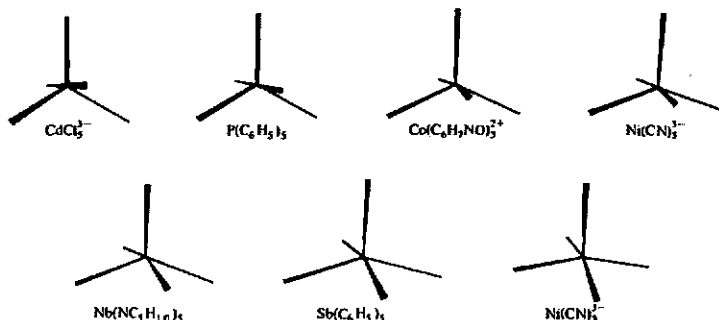
Fig. 6.18 Real five-coordinate molecular structures illustrating intermediates between TBP ( D_{3h} ) on top left to SP ( C_{4v} ) on the bottom right. Note that two different Ni(CN)_5^{2-} polyhedra are found in the unit cell of the Cr(en)_3^{3+} salt. [From Muetterties E. L.; Guggenberger, L. J. J. Am. Chem. Soc. 1974, 96, 1748. Used with permission.]
