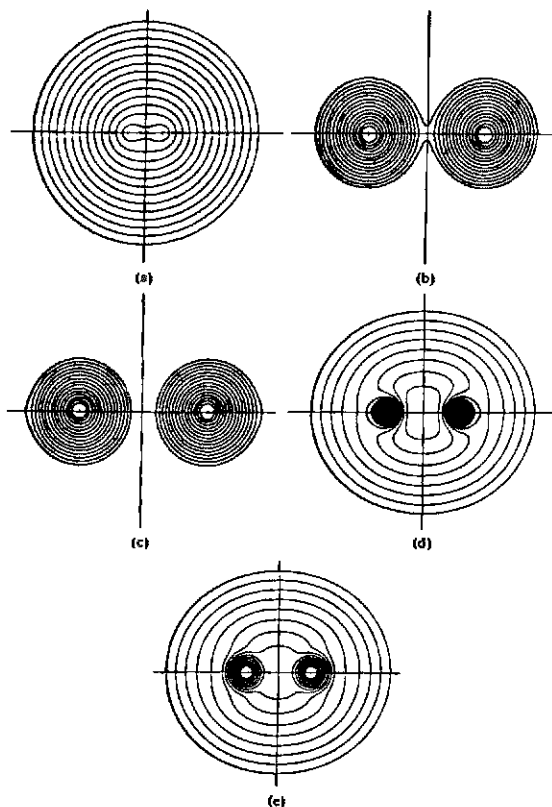
Fig. 5.14 Electron density contours for (a) H_2 ; (b) Li_2 \sigma_{1s} core; (c) Li_2 \sigma_{2s}^* core; (d) Li_2 \sigma_{2s} ; (e) Li_2 , total electron density. [From Wahl, A. C. Science 1966, 151, 961. Reproduced with permission.]
