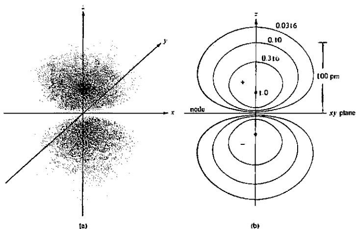
Fig. 2.7 (a) Pictorial representation of the electron density in a hydrogen-like 2p orbital compared with (b) the electron density contours for the hydrogen-like 2p orbital of carbon. Contour values are relative to the electron density maximum. The xy plane is a nodal surface. The signs (+ and -) refer to those of the original wave function. [The contour diagram is from Ogryzlo, E. A.; Porter, G. B. J. Chem. Educ. 1963, 40, 258. Reproduced with permission.]
