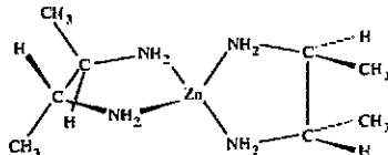
Fig. 3.39 The ( R,R' -2,3-diaminobutane), ( S,S' -2,3-diaminobutane)-zinc(II) ion.
