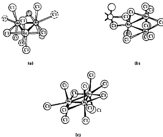
Fig. 16.62 Rhenium(III) clusters: (a) The structural unit present in a Re_3(III) trinuclear cluster. The positions marked \circ are empty in the trihalides in the gas phase but have coordinating groups in other situations. [From Penfold, B. R. In Perspectives in Structural Chemistry ; Dunitz, J. D.; Ibers, J. A., Eds.; Wiley: New York, 1968; Vol. 2, p 71. Reproduced with permission.] (b) The structure of solid (ReCl_3)_3 . [From Colton, F. A.; Mague, J. T. Inorg. Chem. 1964, 3, 1402. Reproduced with permission.] (c) The [Re_3Cl_{12}]^{3-} anion. [From Bertrand, J. A.; Colton, F. A.; Dollase, W. A. Inorg. Chem. 1963, 2, 1166. Reproduced with permission.]
