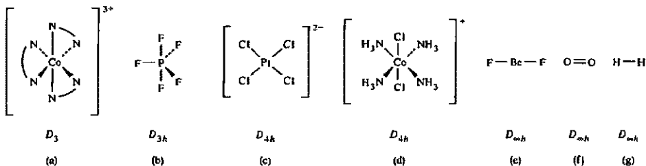
Fig. 3.14 Molecules with D_n , D_{nh} , and D_{\infty h} symmetry: (a) tris(ethylenediamine)cobalt(III) cation, (b) phosphorus pentafluoride, (c) tetrachloroplumate(II) anion, (d) trans -tetraamminedichlorocobalt(III) cation, (e) beryllium difluoride, (f) dioxygen, (g) dihydrogen.
