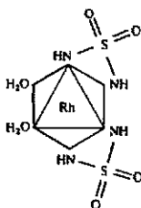
Fig. 12.23 One enantiomer of the cis -diaquabis(sulfamido)rhodate(III) anion.
