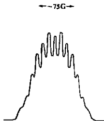
Fig. 11.16 The electron paramagnetic resonance spectrum of \text{K}_2\text{PtCl}_6 in \text{K}_2\text{PtCl}_6 . [From Owen, J. Faraday Disc. Chem. Soc. 1955, 19, 127–134. Reproduced with permission.]
