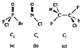
Fig. 3.11 Molecules with low symmetry: (a) phosphoryl bromide chloride fluoride, C_1 ; (b) nitrosyl chloride, C_2 ; (c) the anti conformer of R,S -1,2-dichloro-1,2-difluoroethane, C_1 .
