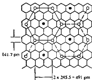
Fig. 16.5 Filling of available hexagonal sites in each layer of graphite; For the limit of C_6K , K = \bullet + \circ ; for C_{12}K , K = \circ only. [From Whittingham, M. S.: Dines, M. B. Surv. Prog. Chem. 1980, 9, 55. Reproduced with permission.]
