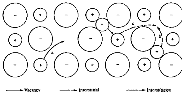
Fig. 7.15 Mechanisms of ionic conduction in crystals with defect structures: (a) vacancy (Schottky defect) mechanism, (b) interstitial (Frenkel defect) mechanism, (c) interstitiality (concerted Schottky-Frenkel) mechanism.
