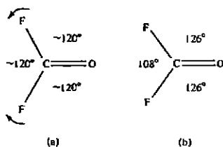
Fig. 6.10 (a) Possible structure of \text{OCF}_2 . Arrows indicate small distortions resulting from electronegativity and size effects. (b) Actual molecular structure of \text{OCF}_2 . Note small \text{FCF} bond angle.
