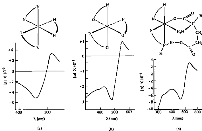
Fig. 12.26 The absolute configurations and ORD spectra of (a) \Lambda - [\text{Co}(\text{en})_3]^{3+} ; (b) \Lambda - [\text{Co}(\text{S-ala})_3] ( S -ala = the anion of S -(L)-alanine); (c) \Lambda - [\text{Co}(\text{en})_2(\text{S-glu})]^- ( S -glu = the dianion of S -(L)-glutamic acid). All of these complexes have the \Lambda or \Delta configuration.
