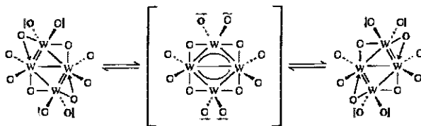
Fig. 16.61 Dynamic intramolecular rearrangement of W_6(O-i-Pr)_{12} . [From Chisholm, M. H.; Clark, D. L.; Hampden-Smith, M. J. J. Am. Chem. Soc. 1989, 111, 574–586. Reproduced with permission.]
