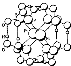
Fig. 15.49 Crystal structure of \text{K}_4[\text{Pt}_2(\mu\text{-P}_2\text{O}_5\text{H}_2)_4] . [From Roundhill, D. M.; Gray, H. B.; Che, C-M. Acc. Chem. Res. 1989, 22, 55-61. Reproduced with permission.]
