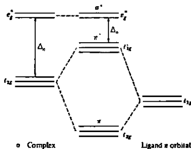
Fig. 11.26 MO diagram for the \pi system of [\text{CoF}_6]^{3-} . Left: MOs for the \sigma system of the complex; right: LGOs of t_{2g} , symmetry; center: MOs after \pi interaction. Note that \Delta_o is diminished by the \pi interaction.
