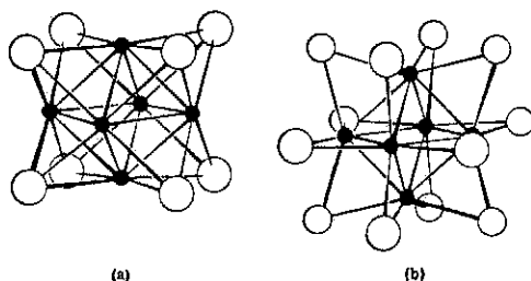
Fig. 16.64 The structure of the \text{Mo}_6\text{Cl}_8^{4+} ion; ● = Mo, ○ = Cl. (b) The structure of the \text{M}_6\text{X}_{12}^{3+} ions; ● = Nb, Ta; ○ = Cl, Br. [From Cotton, F. A. Acc. Chem. Res. 1969, 2, 240. Reproduced with permission.]
