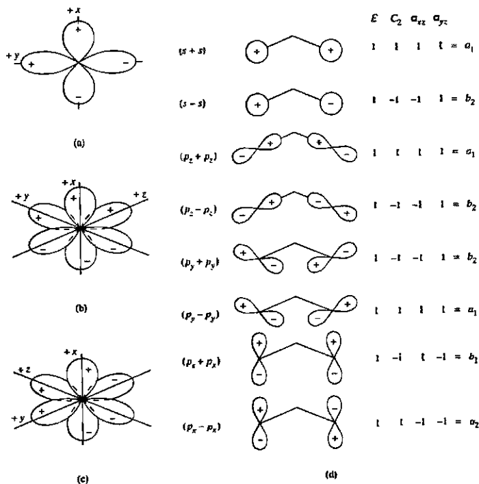
Fig. 5.30 The atomic orbitals of the nitric ion when viewed along the z axis, which is the principal twofold axis of the anion. (a) the p_x and p_y atomic orbitals on nitrogen: The plane of the anion is the yz plane, and the x axis is perpendicular to that plane. (b) The atomic p orbitals of the left-hand oxygen atom. Note that the z axis has been redefined along the O—N bond axis. The x axis is still perpendicular to the plane of the molecule, and the y axis must be mutually perpendicular to x and z . (c) The atomic p orbitals of the right-hand oxygen atom. Again, the z axis has been redefined along the N—O bond axis, and x and y are mutually perpendicular. (d) Group orbitals for the oxygen atoms in \text{NO}_2^- , derived from the 2s and 2p atomic orbitals. The orientations are as shown in parts (b) and (c).
