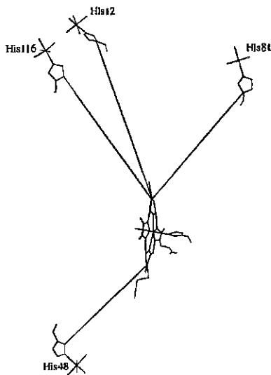
Fig. 13.15 Computer-generated view of the heme group and four ruthenium surface histidines in sperm-whale myoglobin. Closest heme- \sigma -Ru(His) edge-to-edge distances are 14.6 (His48), 19.1 (His81), 20.1 (His116), and 22.1 Å (His12). [From Mayo, S. L.; Ellis, W. R., Jr.; Crutchley, R. J.; Gray, H. B. Science 1986, 233, 948-952. Used with permission.]
