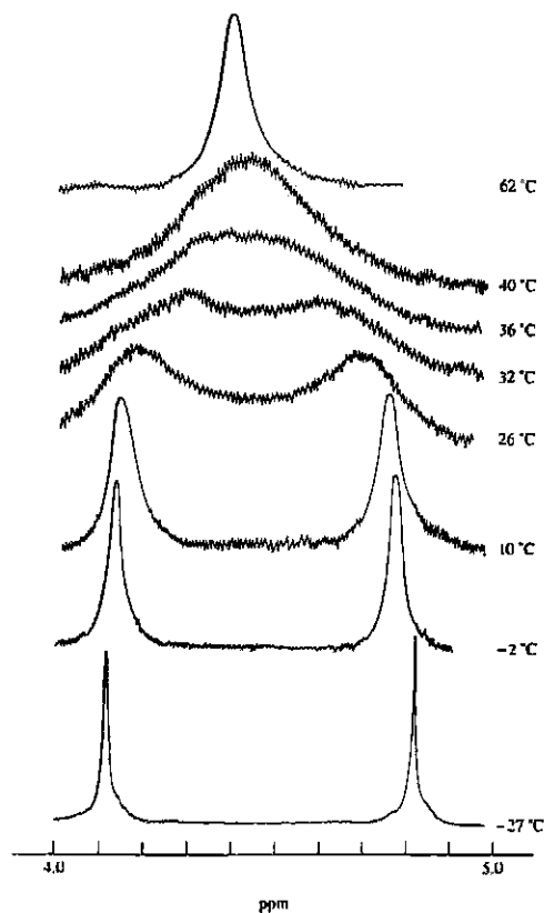
Fig. 15.52 Proton NMR spectra of (\eta^5\text{-C}_5\text{H}_5)_2(\eta^5\text{-C}_5\text{H}_5)_2\text{Ti} from -27 to +62 °C. The separate resonances observed at low temperature for the two types of Cp rings gradually broaden and collapse, giving a single line at 62 °C. [From Cotton, F. A. in Dynamic Nuclear Magnetic Resonance Spectroscopy ; Jackman, L. M., Cotton, F. A., Eds.; Academic: New York, 1975; Chapter 10. Used with permission.]
