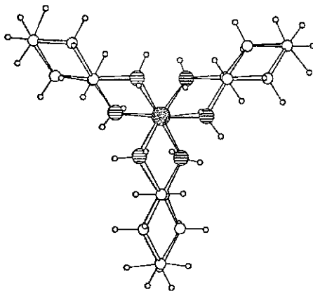
Fig. 12.53 One of two possible enantiomeric solutions to the X-ray crystal structure of the dextrorotatory enantiomer of the tris( R,R - trans -1,2-diaminocyclohexane) cobalt(III) cation, (+)_S^{\text{D}}[\text{Co}(\text{R,R-}i\text{trans-chxn})_3]^{3+} . See Problem 12.31. [Modified from Saito, Y. Inorganic Molecular Dissymmetry ; Springer-Verlag: Berlin, 1979; p 62. Reproduced with permission.]
