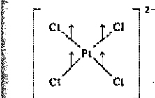
Fig. 3.27 The PtCl_4^{2-} ion with vectors representing orbitals on platinum suitable for out-of-plane \pi bonding.
