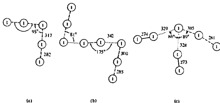
Fig. 17.8 Structures of polyiodide ions: (a) The pentaoidide ion, I_5^- ; (b) the octaoidide ion, I_8^{2-} ; (c) the heptaoidide ion as found in Ph_4PI_7^- . Solid lines represent essentially normal covalent bonds, dashed lines represent weakened or partial bonds, and dotted lines represent very long and weak interactions. Distances in pm.
