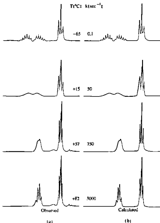
Fig. 15.55 Observed (a) and simulated (b) variable temperature proton NMR spectra of \text{Os}_5(\text{CO})_{10}(\mu, \eta^2\text{-CH}_3\text{CH}_2\text{C}\equiv\text{CCH}_2\text{CH}_3) . The spectrum at -65^\circ\text{C} , characteristic of two equivalent ABX, spin systems, is produced when the movement of the alkyne on the metal surface is slowed sufficiently that it is fixed in one position on the NMR time scale. At +82^\circ\text{C} the alkyne molecule is moving rapidly on the metal surface giving an averaged spectrum in which all methylene protons are equivalent. [From Rosenberg, E.; Brucker-Novak, J.; Gellert, R. W.; Aime, S.; Gobetto, R.; Osetta, D. J. Organomet. Chem. 1989, 365, 163–185. Reproduced with permission.]
