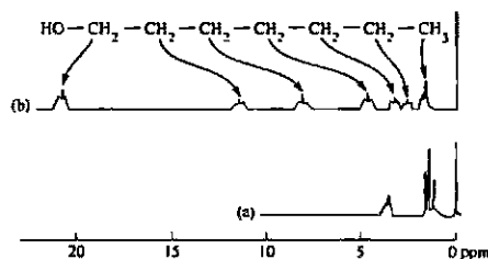
Fig. 14.13 Proton NMR spectra (60 MHz) of 1-heptanol. (a) Spectrum of 0.3 M 1-heptanol in \text{CDCl}_3 . (b) Spectrum of 0.78 molar ratio of tris-(dipivaloyl)europium(III)/1-heptanol in \text{CDCl}_3 . [From Rabenstein, D. L. Anal. Chem. 1971, 43, 1599-1605, as modified by Mayo, B. C. Chem. Soc. Rev. 1973, 2, 49-74. Reproduced with permission.]
