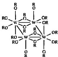
Fig. 16.63 Structure of \text{W}_4(\text{OR})_{16} .
