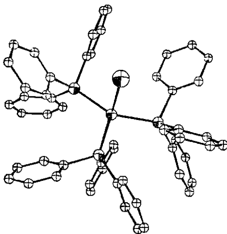
Fig. 15.47 Structure of Wilkinson's catalyst, (\text{Ph}_3\text{P})_3\text{RhCl} . [From Jardine, F. H. Prog. Inorg. Chem. 1981, 28, 63. Reproduced with permission.]
