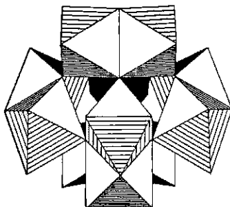
Fig. 16.14 Idealized sketch of the [\text{CeMo}_{12}\text{O}_{42}]^{12-} ion showing the linkage of the \text{MoO}_6 octahedra.
