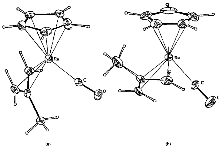
Fig. 15.29 Structures of (a) endo - and (b) exo - \text{Ru}(\eta^3\text{-C}_4\text{H}_7)(\eta^3\text{-C}_3\text{H}_5)(\text{CO}) . [From Hsu, L.-Y.; Nordman, C. E.; Gibson, D. H.; Hsu, W.-L. Organometallics 1989, 8, 241-244. Reproduced with permission.]
