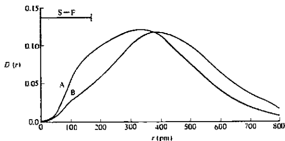
Fig. 18.3 The 3 d orbital distribution functions in d 1 configurations (A) in the 4 D term of P ( s 2 p 3 d 1 ); (B) in the 2 D term of S ( s 2 p 3 d 1 ). Line represents a typical S—F bond length. [Modified from Mitchell, K. A. R. Chem. Rev. 1969, 69, 157. Reproduced with permission.]
