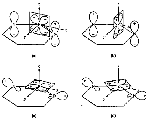
Fig. 16.24 Theory of Craig and Paddock for \pi bonding in phosphazenes: (a) interaction of p_z(N) and d_{xz}(P) ; (b) interaction of p_z(N) and d_{yz}(P) ; (c) interaction of sp^2(N) and d_{xy}(P) ; (d) interaction of sp^2(N) and d_{x^2-y^2}(P) . [From Corbridge, D. E. C. Phosphorus ; Elsevier: Amsterdam, 1978; p 235. Reproduced with permission.]
