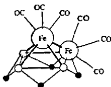
Fig. 16.54 Structure of B 3 H 7 [Fe(CO) 3 ] 2 . [From Gimès, R. N. In Comprehensive Organometallic Chemistry : Wilkinson, G., Stone, F. G. A., Abet, E. W., Eds.; Pergamon: Oxford, 1982; Vol. 1, p 470. Reproduced with permission.]
