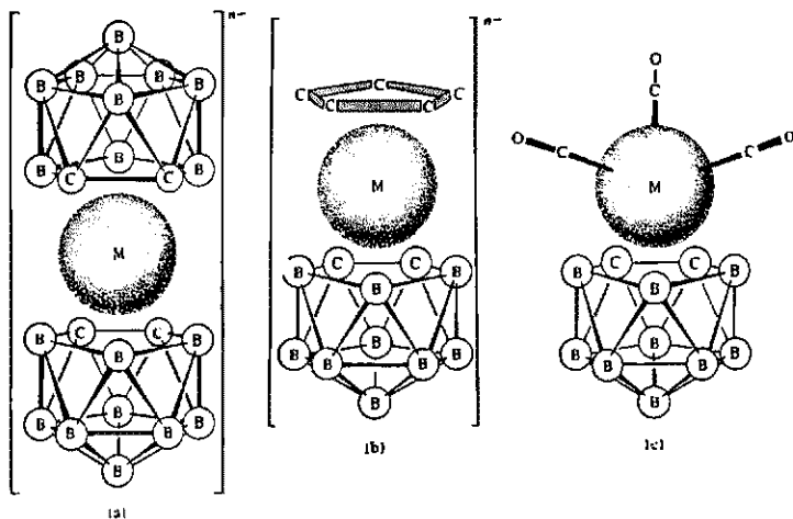
Fig. 16.53 Structures of some carbollene metallocene compounds. (a) Dicarbollyl species: M = \text{Fe} , n = 2 , and M = \text{Co} . n = 1 are isoelectronic with ferrocene and cobaltocenium ion; M = \text{Fe} , n = 1 is isoelectronic with ferrocenium ion; (b) mixed carbollyl-cyclopentadienyl analogue of ferrocene, n = 1 ; (c) mixed carbollyl-carbonyl compound, M = \text{Mn} . Re: (a) and (b) from Hawthorne, M. F.; Andrews, T. D. J. Am. Chem. Soc. 1965, 87, 2496. (c) from Adler, R. G.; Hawthorne, M. F. J. Am. Chem. Soc. 1970, 92, 6174. Reproduced with permission.]
