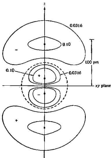
Fig. 2.7 (a) Pictorial representation of the electron density in a hydrogen-like 2p orbital compared with (b) the electron density contours for the hydrogen-like 2p orbital of carbon. Contour values are relative to the electron density maximum. The xy plane is a nodal surface. The signs (+ and -) refer to those of the original wave function. [The contour diagram is from Ogryzlo, E. A.; Porter, G. B. J. Chem. Educ. 1963, 40, 258. Reproduced with permission.]
