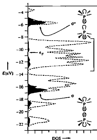
Fig. 7.32 Phosphorus 3p_z orbital contribution (dark area) to the total DOS (dashed line) of the three-dimensional (total) [\text{Mn}_2\text{P}_2]_x^{2-} lattice. The P–P interactions are labeled \sigma and \sigma^* . The square bracket encloses the bands arising principally from the manganese 3d orbitals. [Modified from Hoffmann, R.; Zheng, C. J. Phys. Chem. 1985, 89, 4175–4181. Reproduced with permission.]
