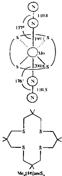
Fig. 15.18 Structure of \text{MoMe}_6[16\text{janeS}_4](\text{N}_2)_2 . Bond lengths are in picometers. [From Yoshida, T.; Adachi, T.; Kaminaka, M.; Ueda, T.; Higuchi, T. J. Am. Chem. Soc. 1988, 110, 4872-4873. Used with permission.]
