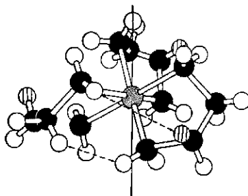
Fig. 12.30 The nb conformer of the \Delta or \iota isomer of iris(diamine)metal complexes. The hatched circles represent the positions of the methyl groups in the propylenediamine complex. For propylenediamine this represents the \Delta\delta\delta\delta or \iota\delta\delta\delta isomer. (Modified from Corey, E. J.; Bailar, J. C., Jr. J. Am. Chem. Soc. 1959, 81, 2620-2629. Reproduced with permission.)
