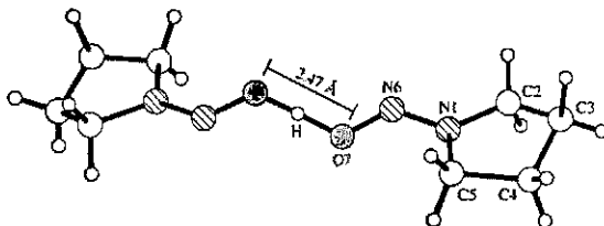
Fig. B.5 Short, symmetrical hydrogen bond in the cation of bis( N -nitrosopyrrolidine)-hydrogen hexafluorophosphate which crystallizes in the monoclinic space group P2_1/c . The hydrogen bonded proton lies on a center of symmetry, with only one of the nitrosopyrrolidine molecules being crystallographically unique. Note that the O—O distance is only 247 pm whereas two times the van der Waals radius of oxygen (Table B.1) is 300 pm. [From Keefe, L. K.; Hrabie, J. A.; Ohannesian, L.; Flippen-Anderson, J. L.; George, C. J. Am. Chem. Soc. 1988, 110, 3701–3702. Reproduced with permission.]
