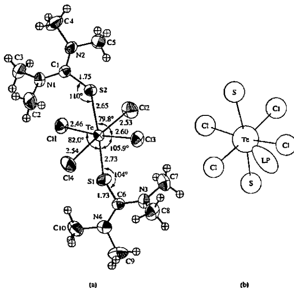
Fig. 6.14 (a) Molecular structure of trans -tetrachlorobis(tetramethylthiurea)tellurium(IV) in the monoclinic form. Note that the line Cl(4)—Te—Cl(2) approximates an axis for a pentagonal bipyramid if it is assumed that a lone pair occupies a position between S(1) and Cl(3) (b). [In part from Esperás, S.; George, J. W.; Husebye, S.; Mikalsen, Ø. Acta Chem. Scand. 1975, 29A, 141–148.]
