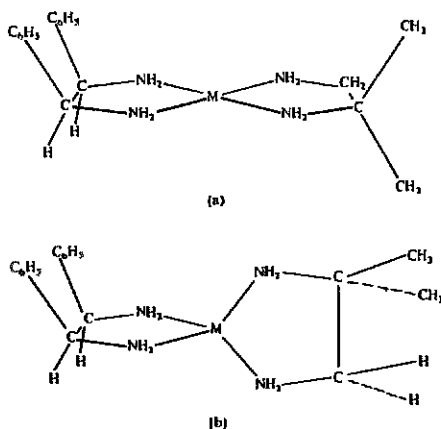
Fig. 12.5 Possible structures of ( meso -stilbediamine) (isobutylendiamine) palladium(II) and platinum(II) complexes: (a) planar structure, optically active; (b) tetrahedral structure, optically inactive.
