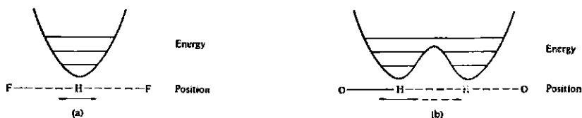
Fig. 15.51 Energy and position of the hydrogen atom in (a) the symmetric \text{HF}_2 system and (b) an unsymmetric \text{O-H}\cdots\text{O} system. In (a) the average position of the hydrogen atom is midway between the fluoride ions. In (b) the positional sketch on the left represents the average position of the hydrogen in the left potential well and the dotted sketch represents the average position for the other potential well. The height of the energy barrier is qualitative and not meant to represent any particular system.
