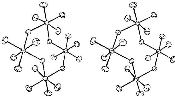
Fig. 7.7 Stereoview of the tetrameric unit of Rh_4F_{20} . The rhodium are at the centers of the octahedra of fluorine atoms. Note bridging fluorine atoms. [From Morrell, B. K.; Zalkin, A.; Tressaud, A.; Bartlett, N. Inorg. Chem. 1973, 12, 2640-2644. Reproduced with permission.]
