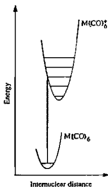
Fig. 11.34 Potential well representations for M(\text{CO})_6 and M(\text{CO})_6^+ , showing origin of vibrational fine structure in PES spectrum. [Modified from Hubbard, J. L.; Lichtenberger, D. L., J. Am. Chem. Soc. 1982, 104, 2132-2138. Used with permission.]
