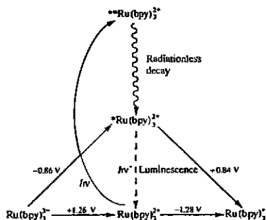
Fig. 13.10 Absorption of blue light by [\text{Ru}(\text{bpy})_3]^{2+} gives [\text{Ru}^*(\text{bpy})_3]^{2+} which relaxes to [\text{Ru}^*(\text{bpy})_3]^{2+} without light emission. [\text{Ru}^*(\text{bpy})_3]^{2+} may emit orange-red light (luminesce) or undergo oxidation or reduction. Standard reduction potentials associated with individual processes are shown in the diagram. [Modified from Juris, A.; Balzani, V.; Barigelli, F.; Campagna, S.; Belser, P.; von Zelewsky, A. Coord. Chem. Rev. 1988, 84, 85–277. Used with permission.]
