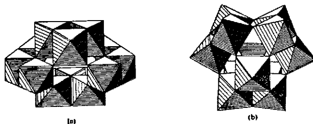
Fig. 16.11 The structures of two apex-shared dodecahedral isopoly anions: (a) the paratungstate B ion, [H_2W_{12}O_{42}]^{10-} ; (b) the metalungstate ion, [H_2W_{12}O_{40}]^{6-} . [From Lipscomb, W. N. Inorg. Chem. 1965, 4, 132. Reproduced with permission.]
