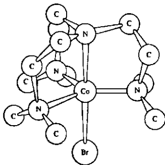
Fig. 12.10 Molecular structure of bromotrakis(2-dimethylaminoethyl)aminocobalt(II) cation in [\text{CoBr}(\text{Me}_6\text{tren})]\text{Br} . [From Di Vaira, M.; and Orioli, P. L. Inorg. Chem. 1967, 6, 955. Reproduced with permission.]
