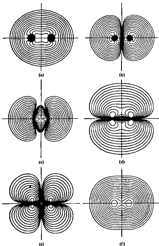
Fig. 5.15 Electron density contours for various orbitals in the O 2 molecule. (a) \sigma_g^2 ; (b) \sigma_u^2 ; (c) \sigma_g^2 ; (d) \pi_u^2 ; (e) \pi_g^2 ; (f) total electron density. [From Wahl, A. C. Science 1966, 151, 961. Reproduced with permission.]
