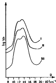
Fig. 11.48 Electronic spectra of \text{Rb}_2\text{Na}[\text{TiCl}_6] (I), \text{Cs}_2\text{K}[\text{TiCl}_6] (II), and \text{Rb}_1[\text{TiCl}_6] (III). [From Ameis, R.; Kremer, S.; Reinen, D. Inorg. Chem. 1985, 24, 2751-2754. Used with permission.]
