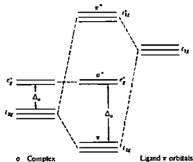
Fig. 11.27 MO diagram for the \pi system of an octahedral complex with acceptor ligands such as CO, \text{PR}_3 , or \text{SR}_2 . Note that the \pi interaction in this case increases \Delta_o .
