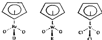
Fig. 15.39 Cyclopentadienyl complexes in which the metal is in a high oxidation state.
