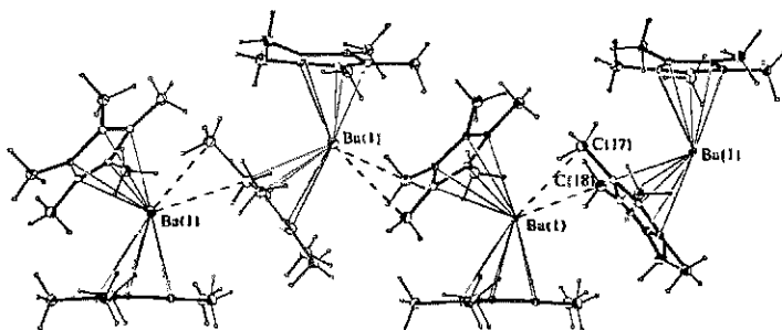
Fig. 15.36 Solid-state structure of (\text{Me}_5\text{C}_5)_2\text{Ba} . Metalloene units are arranged in quasipolymeric chains and a ring-Ba-ring tilt of 131^\circ is observed. Lines connecting Ba and methyl groups indicate the shortest intermolecular contacts. [From Williams, R. A.; Hanusa, T. P.; Huffman, J. C. J. Chem. Soc. Chem. Commun. 1988, 1045-1046. Reproduced with permission.]
