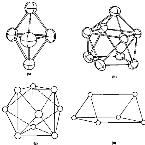
Fig. 16.66 Some representative Zintl ions: (a) \text{Pb}_7^{4-} , (b) \text{Sn}_9^{4-} , (c) \text{Bi}_9^{3+} , (d) \text{Te}_6^{4+} .
