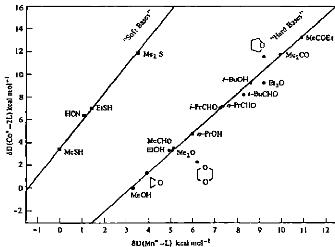
Fig. 9.8 Comparison of relative ligand dissociation energies for Mn^+ and Co^+ . Zero points for the scales have been arbitrarily chosen. Note that for the soft ligands, MeSH, HCN, EtSH, and Me_2S , the data points lie above and to the left of those for the oxygen bases. This indicates relatively stronger hard-hard bonding ( O-Mn^+ ) or soft-soft bonding ( S-Co^+ ), or both. (Modified from Jones, R. W.; Staley, R. H. J. Phys. Chem. 1982, 86, 1387. Reproduced with permission.)
