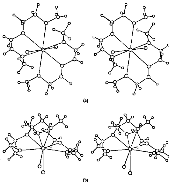
Fig. 12.39 Stereoviews of the structure of (a) \text{trans-SmI}_2[\text{O}(\text{CH}_2\text{CH}_2\text{OCH}_3)_2]_2 and (b) \text{cis-SmI}_2[\text{O}(\text{CH}_2\text{CH}_2\text{OCH}_3)_2]_2 . [From Sen, A.; Chebott, V.; Rheingold, A. L. Inorg. Chem. 1987, 26, 1821–1823. Reproduced with permission.]
