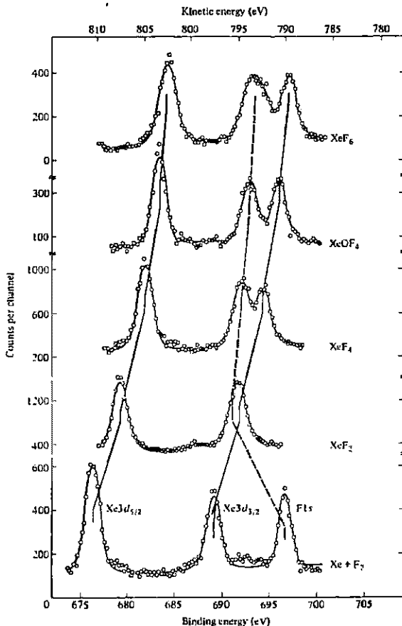
Fig. 17.13 Photoelectron spectra of Xe, \text{F}_2 , \text{XeF}_2 , \text{XeF}_4 , \text{OXeF}_4 , and \text{XeF}_6 . [From Carroll, T. X.; Shaw, R. W., Jr.; Thomas, T. D.; Kindle, C.; Bartlett, N. J. Am. Chem. Soc. 1974, 96, 1989. Reproduced with permission.]
