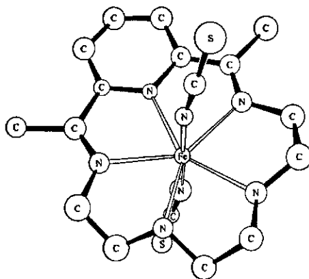
Fig. 12.32 Molecular structure of the seven-coordinate complex of iron involving 2,13-dimethyl-3,6,9,12,18-pentaazabicyclo-[12.3.1]-octadeca-(18),2,12,14,16-pentaene and two axial \text{SCN}^- ligands. Hydrogen atoms omitted. [From Fleischer, E.; Hawkinson, S. J. Am. Chem. Soc. 1967, 89, 720-721. Reproduced with permission.]
