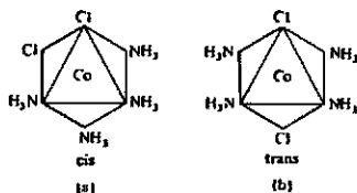
Fig. 12.18 Examples of cis and trans octahedral isomers: (a) cis -tetraamminedichlorocobalt(III), Werner's violeo complex, and (b) trans -tetraamminedichlorocobalt(III), Werner's praseo complex.
