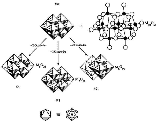
Fig. 16.10 The structures of edge-shared isopoly anions showing their relation to the M_{10}O_{28} structure: (a) M = V ; (b) M = Mo ; (c) M = Mo ; (d) M = Nb, Ta . [From Kepert, D. L. Inorg. Chem. 1969, 8, 1556, and Duy, V. W.; Klemperer, W. G.; Maltbie, D. J. J. Am. Chem. Soc. 1987, 109, 2991-3002. Reproduced with permission.]
