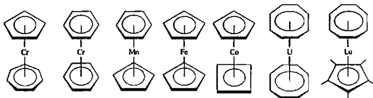
Fig. 15.31 Some examples of known metalloenes containing four-, five-, six-, seven-, and eight-membered rings.
