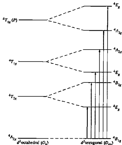
Fig. 11.45 Alteration of energy levels for a d^3 ion as the symmetry of its environment changes from octahedral ( O_h ) to tetragonal ( D_{4h} ).
