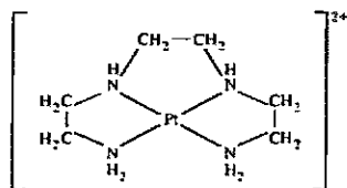
4. tetradentate chelation
