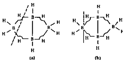
Fig. 16.43 Bonding and structure of tetraborane, B_4H_{10} . [From Muetterties, E. L. The Chemistry of Boron and Its Compounds ; Wiley: New York, 1967. Reproduced with permission.]
