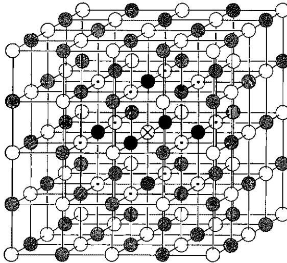
Fig. 4.7 An extended lattice of sodium chloride. Starting with the sodium ion marked \odot , there are six nearest neighbors ( \bullet ), twelve next nearest neighbors ( \ominus ), eight next, next nearest neighbors (darkly shaded), and so on.
