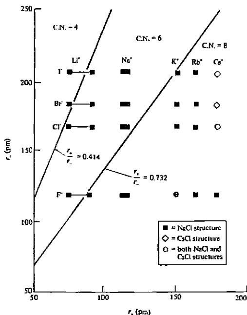
Fig. 4.18 Actual crystal structures of the alkali halides (as shown by the symbols) contrasted with the predictions of the radius ratio rule. The figure is divided into three regions by the lines r_a/r_c = 0.414 and r_a/r_c = 0.732 , predicting coordination number 4 (wurtzite or zinc blende, upper left), coordination number 6 (rock salt, NaCl, middle), and coordination number 8 (CsCl, lower right). The crystal radius of lithium, and to a lesser extent that of sodium, changes with coordination number, so both the radii with C.N. = 4 (left) and C.N. = 6 (right) have been plotted.
