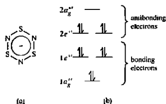
Fig. 16.32 (a) Structure of S_3N_3^- and (b) qualitative molecular orbital diagram. [From Chivers, T.; Oakley, R. T. Top. Curr. Chem. 1982, 102, 117. Reproduced with permission.]
