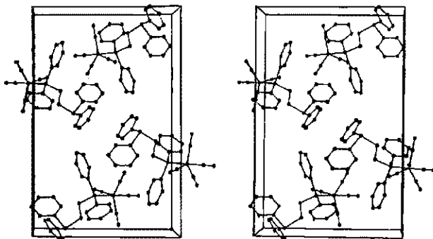
Fig. 3.38 Stereoview of the unit cell of Fe(CO)_4(\eta^1\text{-}PPh_2CH_2CH_2PPh_2) . [From Keiser, R. L.; Rheingold, A. L.; Hamerski, J. J.; Castle, C. K. Organometallics 1983, 2, 1635–1639. Reproduced with permission.]
