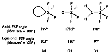
Fig. 6.11 Molecular structures of (a) sulfur tetrafluoride; (b) thionyl tetrafluoride; (c) methylene sulfur tetrafluoride; the hydrogen atoms are in a vertical plane with the axial fluorine atoms.
