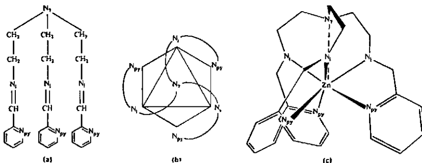
Fig. 12.35 [M(\text{py}_3\text{tren})]^{2+} complexes: (a) The \text{py}_3\text{tren} ligand: \text{N}(\text{CH}_2\text{CH}_2\text{N}=\text{CHC}_6\text{H}_4\text{N})_3 ; the nitrogen atoms are labeled \text{N}_{\text{py}} , the pyridine nitrogen, \text{N}_{\text{pyy}} , the imine nitrogen, and \text{N}_7 , the seventh or unique nitrogen atom; (b) a diagrammatic representation of the [M(\text{py}_3\text{tren})]^{2+} complex, viewed down the threefold axis; (c) the molecular structure of the zinc(II) complex, viewed perpendicular to the threefold axis. [Courtesy of E. C. Lingafelter.]
