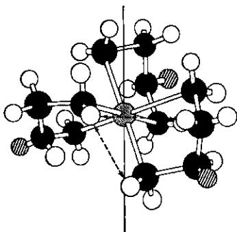
Fig. 12.29 The tel conformer of the \Lambda or D enantiomer of tris(diamine) metal complexes. The hatched circles represent the positions of the methyl groups in the propylenediamine complex. For propylenediamine, this represents the \Lambda\delta\delta\delta or D\delta\delta\delta isomer. [Modified from Corey, E. J.; Bailar, J. C., Jr. J. Am. Chem. Soc. 1959, 81, 2620-2629. Reproduced with permission.]
