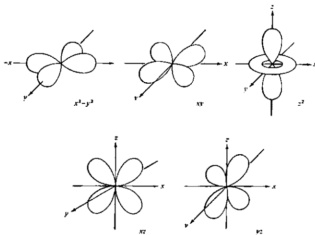
Fig. 11.3 Spatial arrangement of the five d orbitals.
