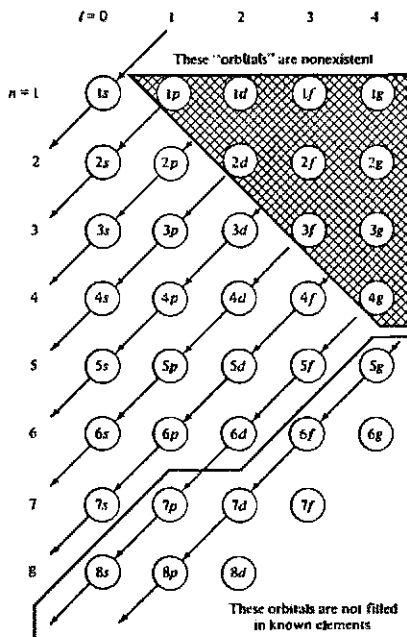
Fig. 2.10 Mnemonic for determining the order of filling of orbitals (approximate). [Adapted from Moeller, Inorganic Chemistry , Wiley: New York, 1952. Reproduced with permission.]
