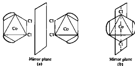
Fig. 12.21 (a) Optical isomers of cis -dichlorobis(ethylenediamine)cobalt(III) ion ( violeto salt). (b) trans -Dichlorobis(ethylenediamine)cobalt(III) ion ( ptaseo salt) showing one internal plane of symmetry (there are two others perpendicular to the one shown).
