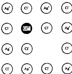
Fig. 7.11 Schottky defect (cation vacancy) induced and balanced by the presence of a higher valence cation. [Hannay, N. B. Solid-State Chemistry ; Prentice-Hall: Englewood Cliffs, NJ, 1967. Reproduced with permission.]
