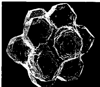
Fig. 3.35 Scanning electron micrograph of a cluster of quasicrystals of \text{Al}_6\text{CuLi}_3 . [Courtesy of B. Dubost and P. Sainfort, Pechiney, France.]
