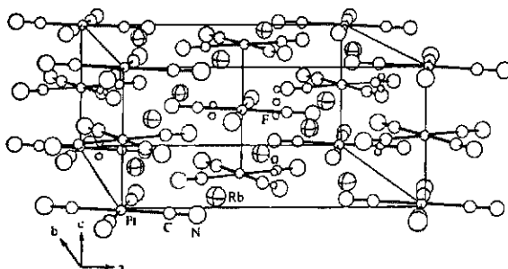
Fig. 16.8 Perspective view of the unit cell of \text{Rb}_2[\text{Pt}(\text{CN})_4](\text{FHF})_{10.40} . One-dimensional chains of staggered [\text{Pt}(\text{CN})_4]^{2-} ions occupy the corners and center of the unit cell. The triad of small circles represents the partially occupied positions of the \text{FHF}^- ions. Note the very short Pt—Pt distance [279.8 pm]. [From Schultz, A. J.; Coffey, C. C.; Lee, G. C.; Williams, J. M. Inorg. Chem. 1977, 6, 2129. Reproduced with permission.]
