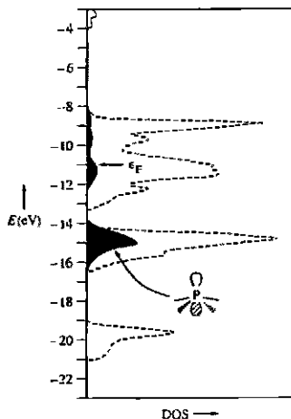
Fig. 7.31 Phosphorus 3p_z orbital contribution (dark area) to the total DOS (dashed line; cf. Figs. 7.29 and 7.30) of the [\text{Mn}_2\text{P}_2]_x^{2-} layer. [Modified from Hoffmann, R.; Zheng, C. J. Phys. Chem. 1985, 89, 4175–4181. Reproduced with permission.]
