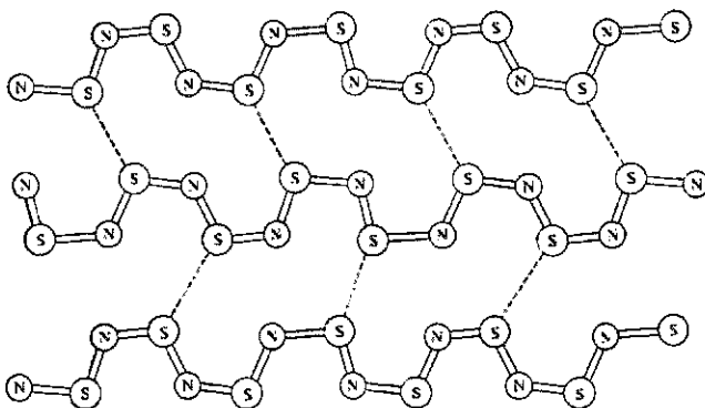
Fig. 16.6 (SN) n chains in one layer of polymeric sulfur nitride. [From MacDiarmid, A. G.; Mikulski, C. M.; Saran, M. S.; Russo, P. J.; Cohen, M. J.; Bright, A. A.; Garito, A. F.; Heeger, A. J. In Compounds with Unusual Properties ; King, R. B., Ed.; Advances in Chemistry Series 150, American Chemical Society: Washington, DC, 1976. Reproduced with permission.]
