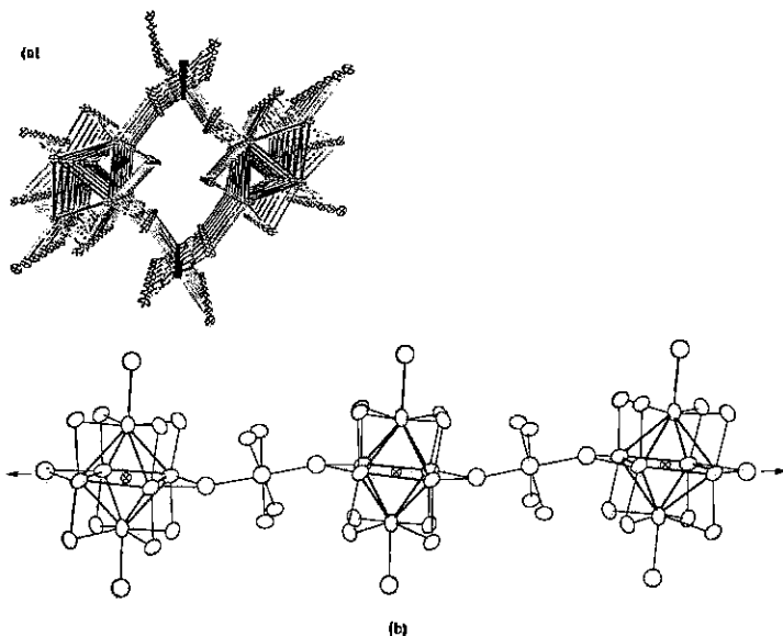
Fig. 16.69 (a) The structure of “ \text{Sc}_5\text{Cl}_{18} ” as it was first reported with stacked \text{Sc}_5 octahedra (black bonds) and bridging stacked \text{ScCl}_6 octahedra (black atoms and white bonds). The poorly scattering nitrogen atoms are not located. (b) The correct structure of \text{Sc}_5\text{Cl}_{18}\text{N} showing \text{Sc}_5\text{Cl}_{12}\text{N} units bridged by \text{ScCl}_6 . The interstitial nitrogen atoms lie at the center of the \text{Sc}_5 octahedra. Part (a) shows several layers of a pair of these chains. If the nitrogen atoms were shown in (a) they would be stacked in the center of the two columns of stacked black parallelograms, \infty . [From Hwu, S.-J.; Dudis, D. S.; Corbett, J. D. Inorg. Chem. 1987, 26, 469–473. Reproduced with permission.]
