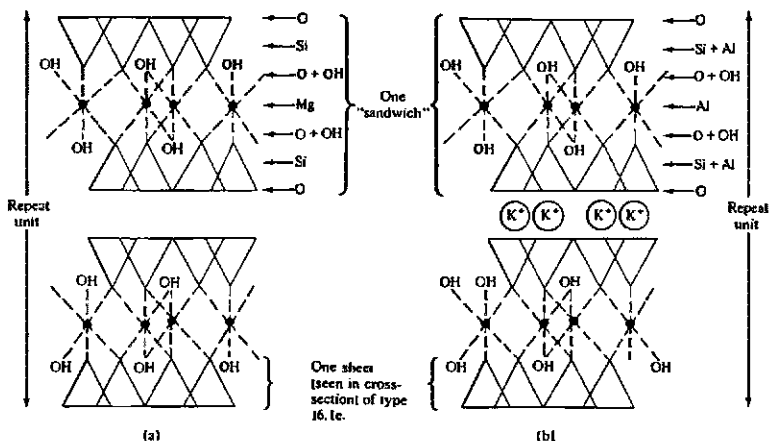
Fig. 16.3 Layered silicate structures: (a) talc, Mg_3(OH)_2(Si_4O_{10}) ; (b) muscovite mica, KAl_2(OH)_2Si_3AlO_{10} . [Note: (1) Electroneutrality is maintained by balance of K(II) , Mg(II) , Al(III) , and Si(IV) . (2) The repeating layers in muscovite are bound together by the K^+ cations.] [From Adams, D. M. Inorganic Solids ; Wiley: New York, 1974. Reproduced with permission.]
