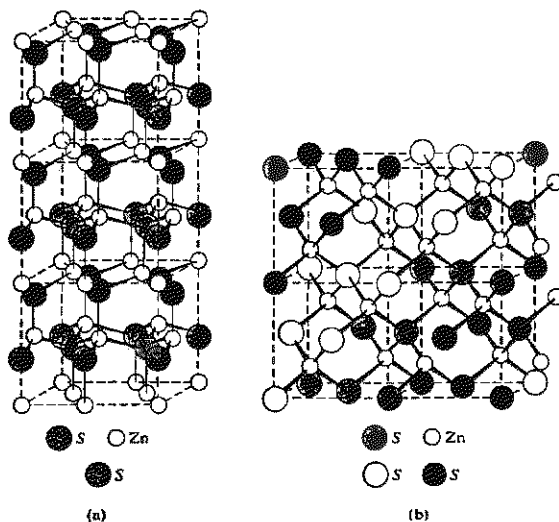
Fig. 4.15 (a) The structure of wurtzite. The sulfide ions form a hcp array with A (gray) and B (black) alternating layers (Cf. Fig. 4.13a). (b) The structure of zinc blende. The sulfide ions form a ccp array with A (white), B (black), and C (gray) layers. (Cf. Figs. 4.13b and 4.14.) Note that in both structures the zinc atoms ( small white circles ) occupy tetrahedral holes.
