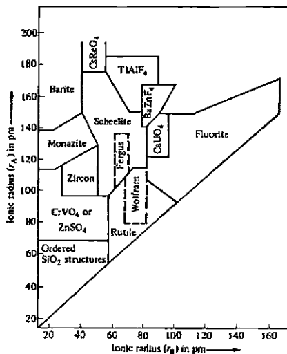
Fig. 7.5 Composite structure field map for \text{ABX}_4 structures, X = F or O. [From Muller, O.; Roy, R. The Major Ternary Structural Families ; Springer-Verlag: New York, 1974. Reproduced with permission.]
